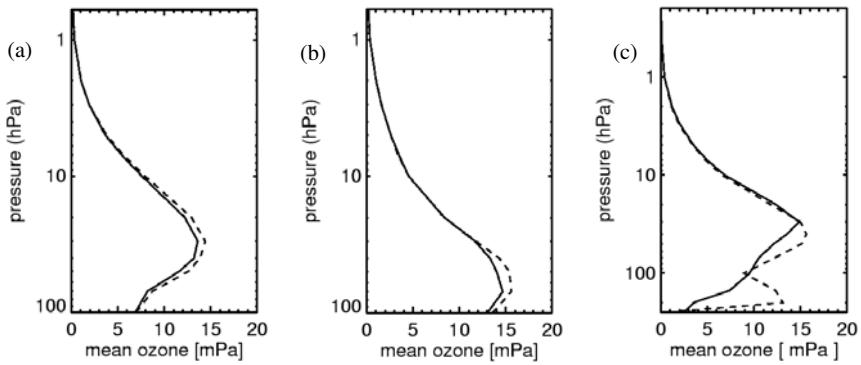
Figure 1. Comparison of the mean of coincident (see text for tolerance) MIPAS ozone profiles (dashed) in December 2002 against (a) HALOE data, 25°–48°N (79 profiles), (b) POAM data, 63.5°–64.5°N (31 profiles), and (c) SBUV assimilation, 30°–60°N (2075 profiles). Note that the vertical range on (c) is greater than on the other two panels.
