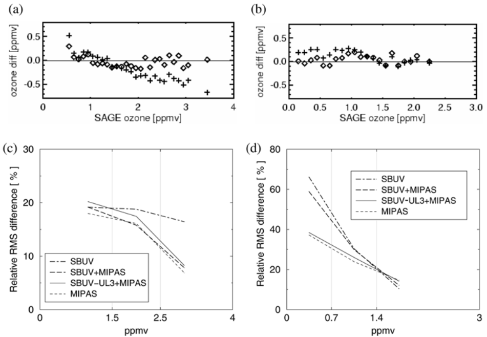
Figure 16. Comparison of assimilated ozone with SAGE data in northern midlatitudes: mean analysis-minus-SAGE differences in bins of 0.1 ppmv at (a) 70 hPa for SBUV (+) and SBUV + MIPAS ( \diamond ) analyses, and (b) 100 hPa for SBUV + MIPAS (+) and SBUV-UL3 + MIPAS ( \diamond ) analyses, and relative r.m.s. differences between SAGE and the four assimilation experiments for low, medium, and high ozone bins (see text for details) at (c) 70 hPa and (d) 100 hPa.
