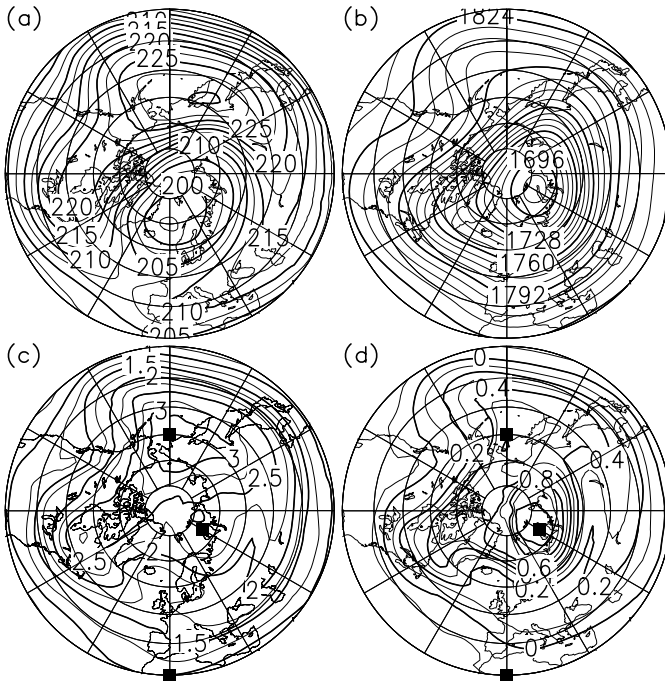
Figure 9. Polar stereographic plots, showing monthly mean fields at 70 hPa in January 2003, north of 30°N: (a) temperature, with contour interval 2.5 K, (b) geopotential height, with interval 8 gpdm, (c) ozone from the SBUV + MIPAS assimilation, with interval 0.25 ppmv, and (d) ozone difference (SBUV + MIPAS minus the SBUV assimilation), with interval 0.1 ppmv. The points marked on (c) and (d) are 75°N 60°E, 60°N 180°E and 30°N 0°E.
